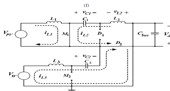
M_1 on, M_2 off
