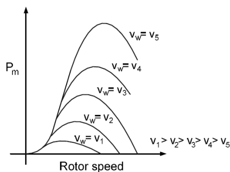
Figure 8: Power Curves for a typical wind turbine
