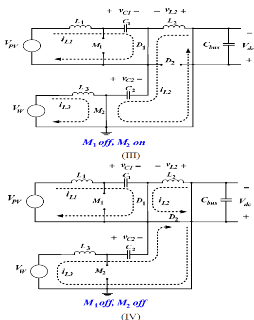
Figure 5 (I-IV): switching states within a switching cycle
