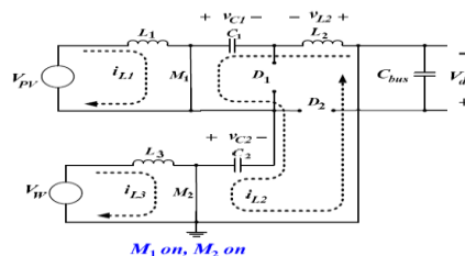
M_1 on, M_2 on
