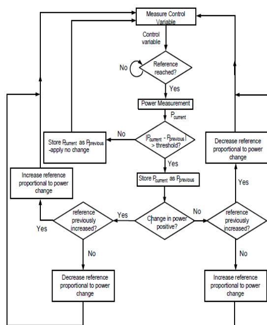
Figure 12: General MPPT Flow Chart for wind and PV
