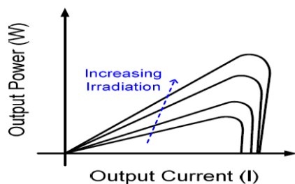
Figure 11: PV cell power characteristics
