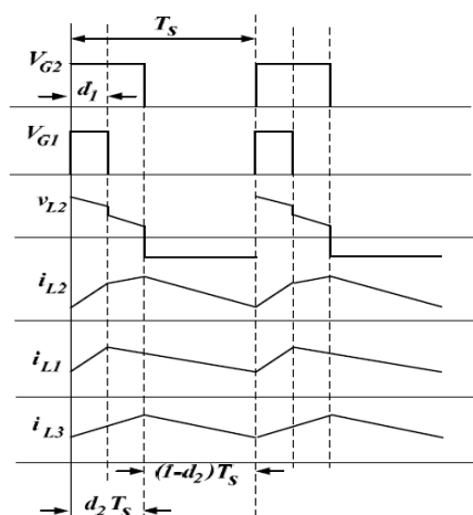
Figure 6: Proposed circuit inductor waveforms
