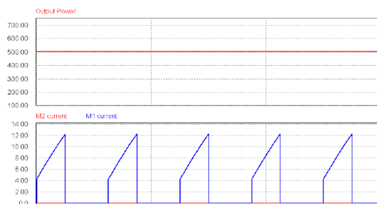
Figure 13 : Individual operation with only PV source (Cuk operation)
