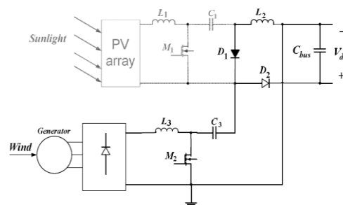
Figure 3: Only wind source is operational (SEPIC)
