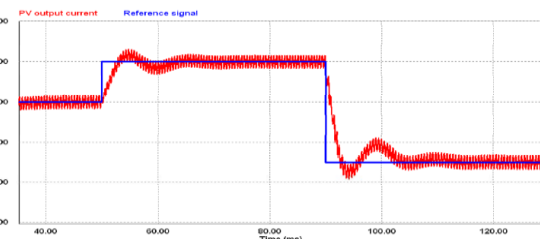
Figure 16 : Solar MPPT – PV output current and reference current signal (Cuk operation)
