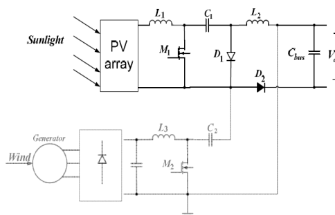
Figure 4: Only PV source is operation (Cuk)
