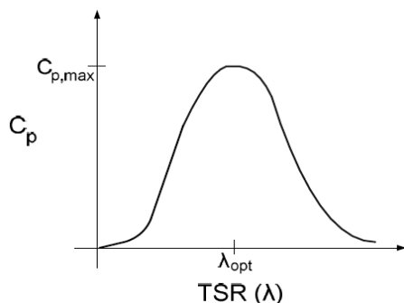
Figure 7: Power Coefficient Curve for a typical wind turbine.
