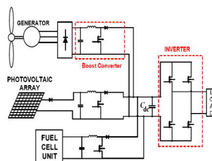
Figure 1: Hybrid system with multi-connected boost converter
