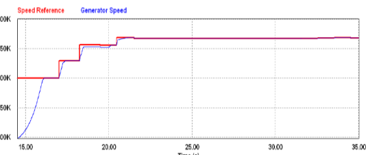
Figure 17: Wind MPPT – Generator speed and reference speed signal (SEPIC operation)
