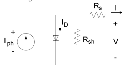
Figure 9: PV cell equivalent circuit
