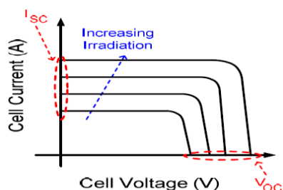
Figure 10: PV cell voltage-current characteristic
