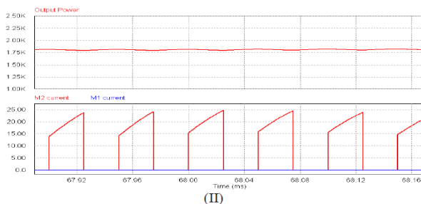
Figure 14 : Individual operation with only wind source (SEPIC operation) (I) The injected three phase generator current; (II) Top: Output power, Bottom: Switch currents (M1 and M2)
